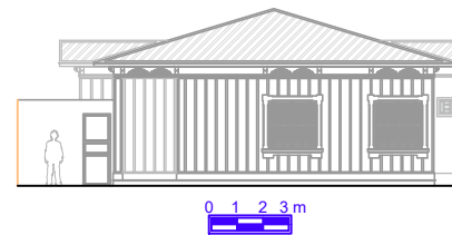
Elevation 03
