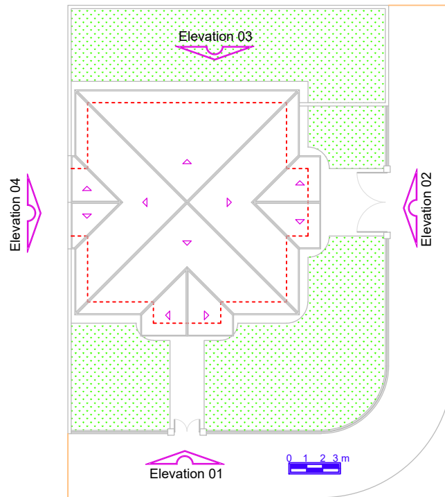
Roof Plan
